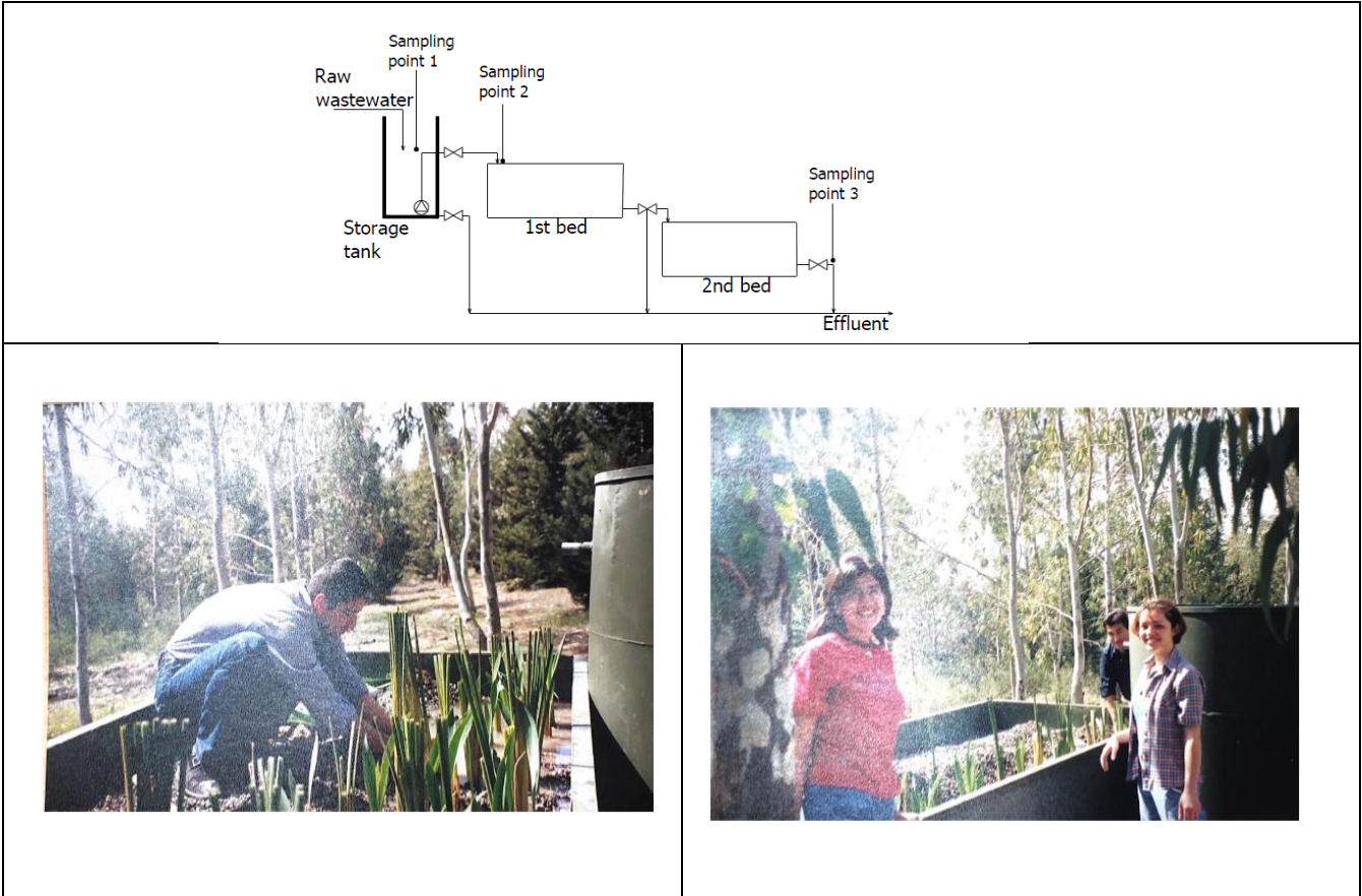
Figure 24. Pilot scale watery area system
